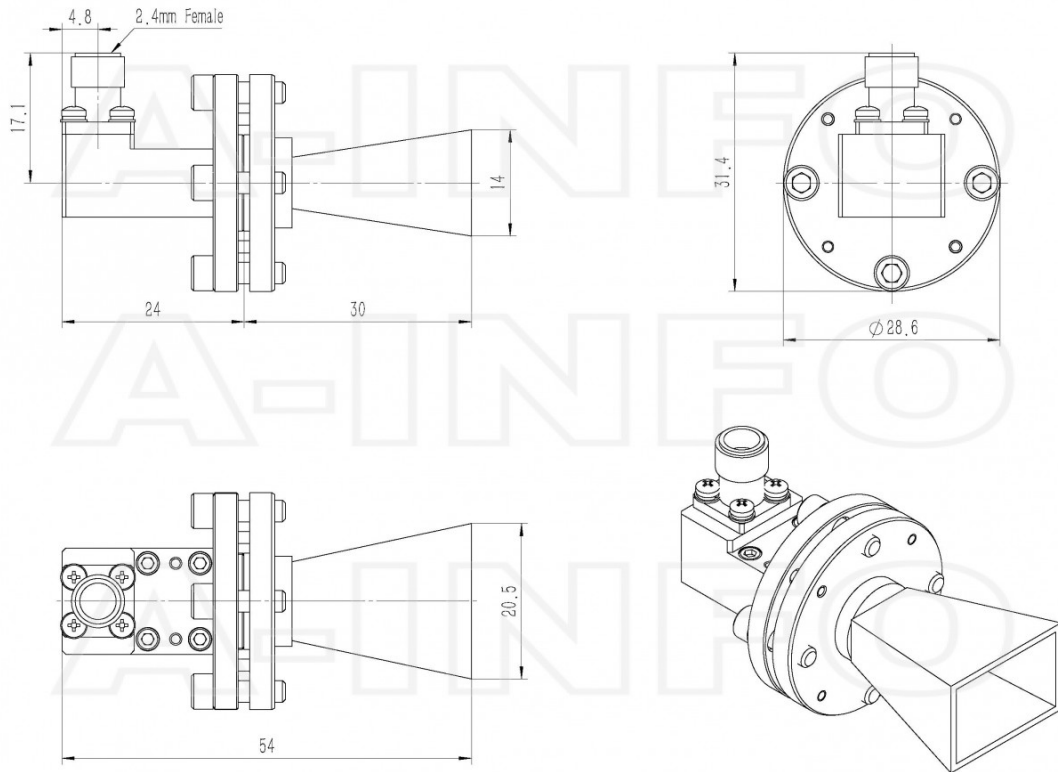
2.4mm-Female Output (P/N: LB-22-15-C-2.4F)
